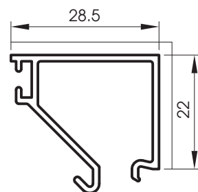
5055 Parclose clipable 28.5 mm
