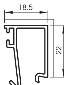
5053 Parclose clipable 18.5 mm
