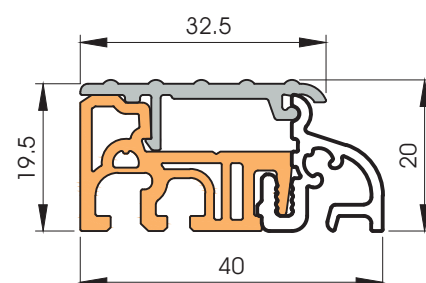
P5057 Seuil RPT portes repliables
