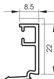
5051 Parclose clipable 8.5 mm
