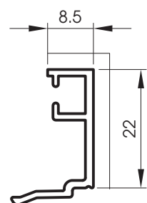
5051L Parclose laquable clipable 8.5 mm
