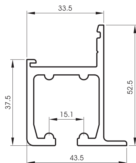
P5055 Rail haut porte repliable
