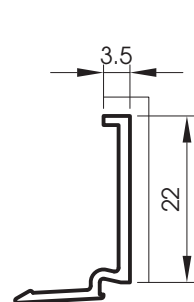
5050 Parclose clipable 3.5 mm
