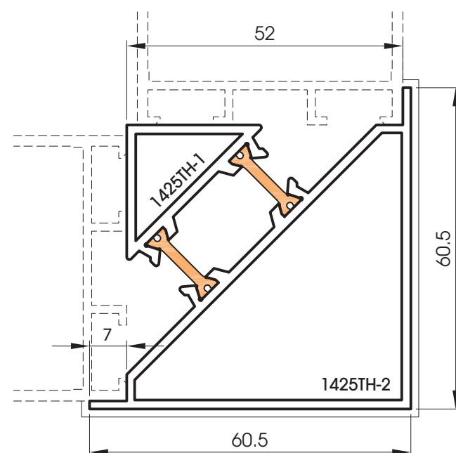
1425TH Angle 53.5 x 53.5 mm
