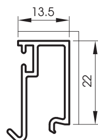
5052 Parclose clipable 13.5 mm
