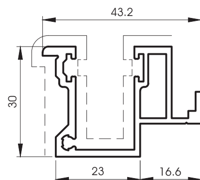
P5056 Rail bas portes repliables
