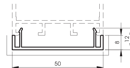
5979 Closir 50
