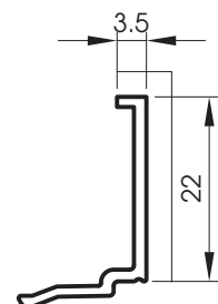
5050L Parclose laquable clipable 3.5 mm
